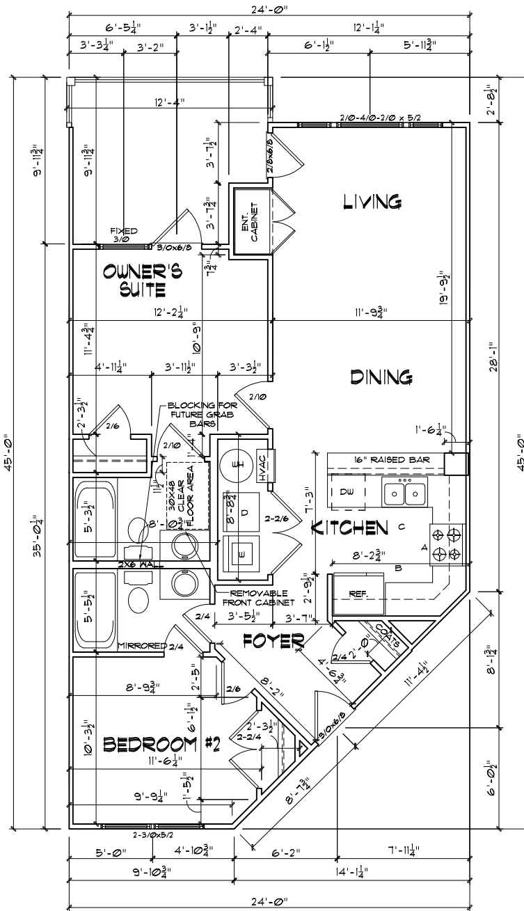
UNIT TYPE 2 FIRST FLOOR PLAN SCALE: 1/8"=1'-0"
