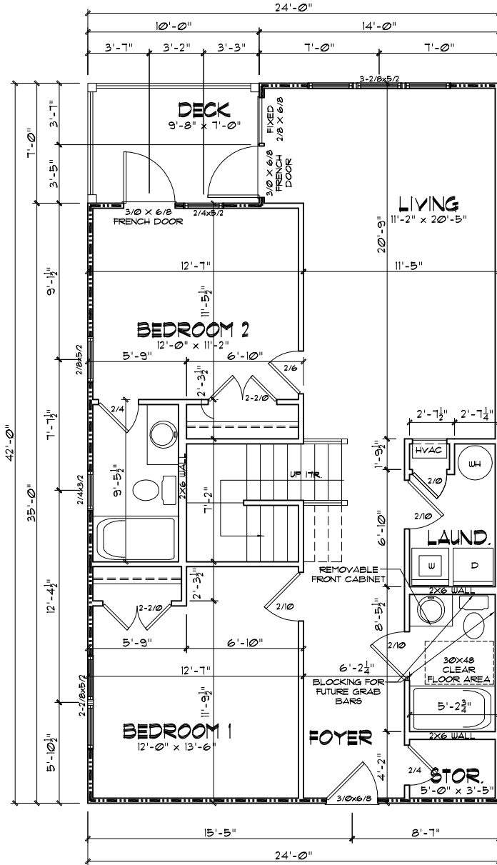
UNIT TYPE 4 FIRST FLOOR PLAN SCALE: 1/8" = 1'-0"
