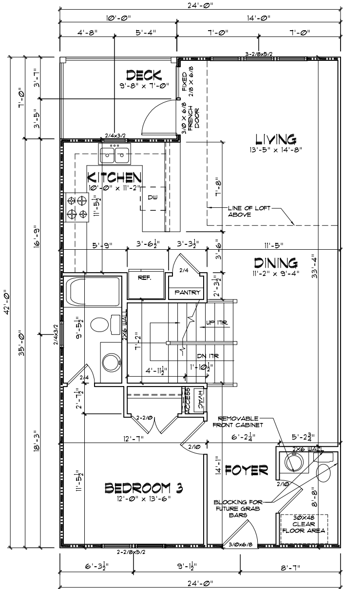
UNIT TYPE 4 SECOND FLOOR PLAN SCALE: 1/8" = 1'-0"
