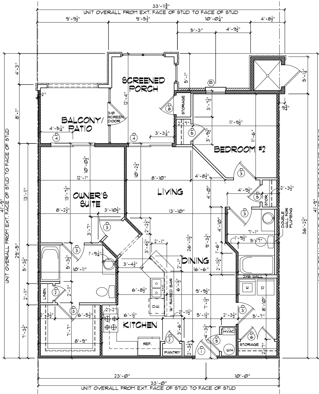
FIRST FLOOR UNIT PLAN UNIT TYPE U0055 SCALE: 1/4"=1'-0" FRONT/SIDE UNIT
